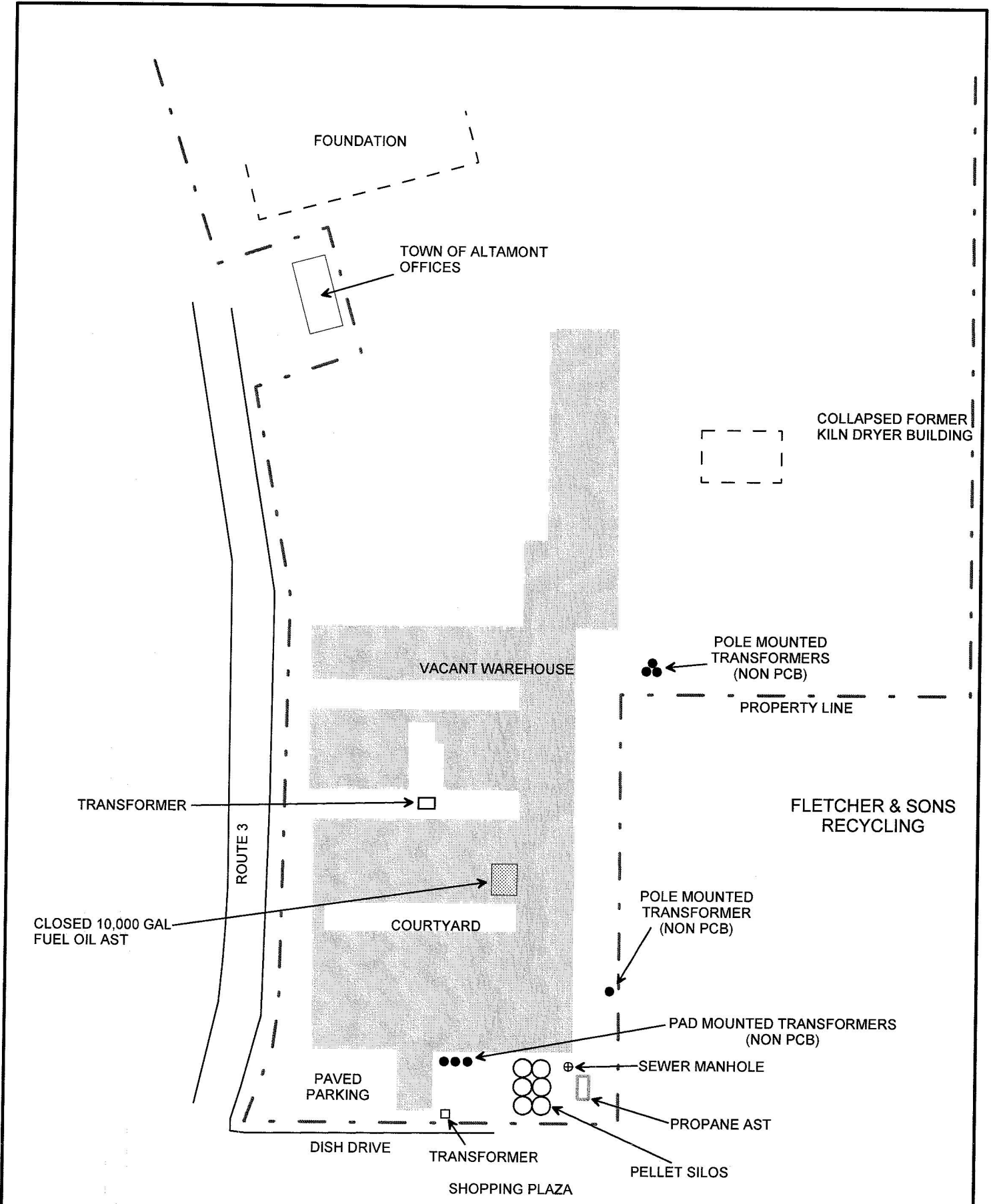
FIGURE 3: SITE SCHEMATIC FORMER OVAL WOOD DISH FACILITY ROUTE 3 TUPPER LAKE, NY
